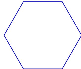
Regular Hexagon
