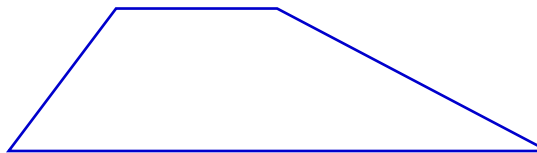
Trapezoid
