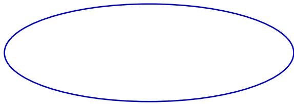
Ellipse
