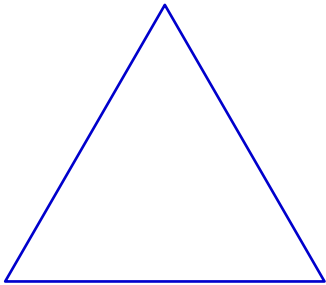
Equilateral Triangle
